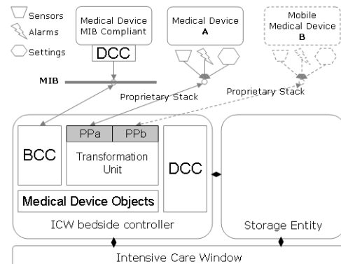
Fig. 1. Intensive Care Window architecture
