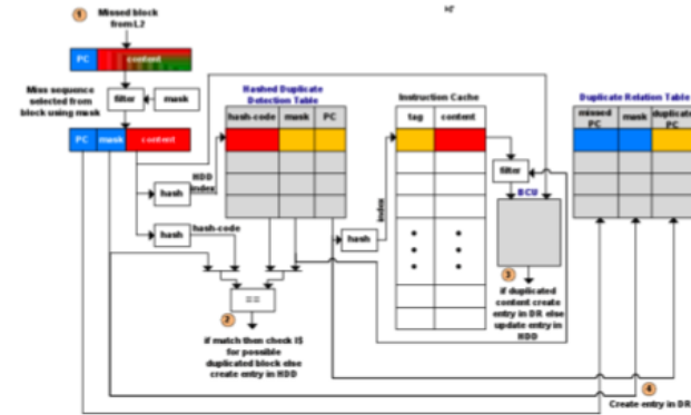
Computer architecture
